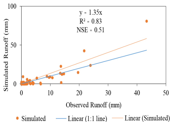
Figure 10. Daily runoff volumes simulated from Catchment 104 under bare fallow cover with observed runoff scaled by a factor of 40%
